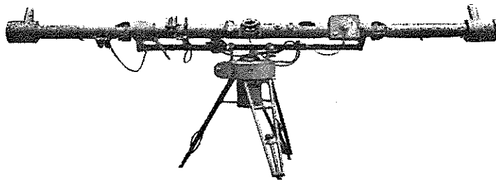
Stereotelemeter.
